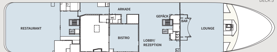
DECK 5
